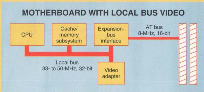
Figure A: The CPU, memory/cache subsystem, and expansion bus interface make up the heart of the motherboard. They are connected by a high-speed synchronous local bus that runs at the speed of the CPU. With this architecture, PC makers are realizing speeds that are four to 16 times faster than those of motherboards built around asynchronous buses, such as ISA, EISA, or Micro Channel.
